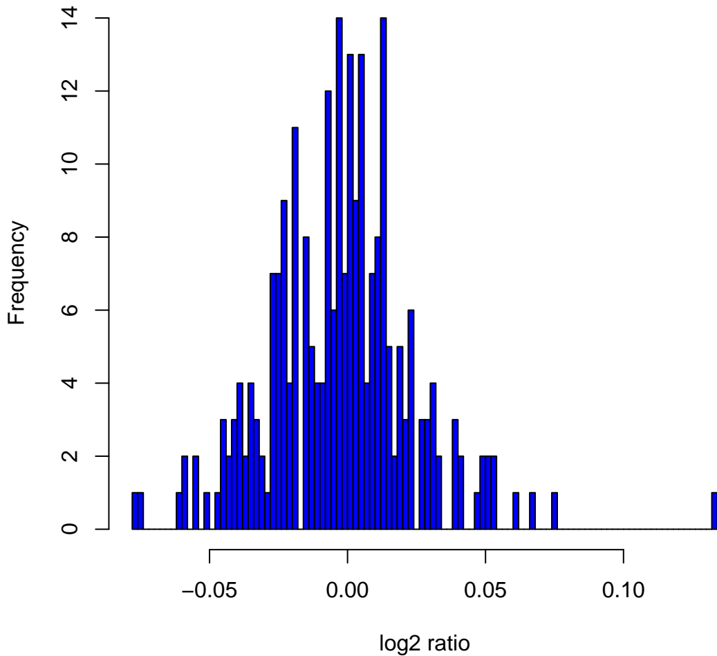
Histogram of log 2 ratios in 270 HapMap samples at clone Chr12tp-7C4
