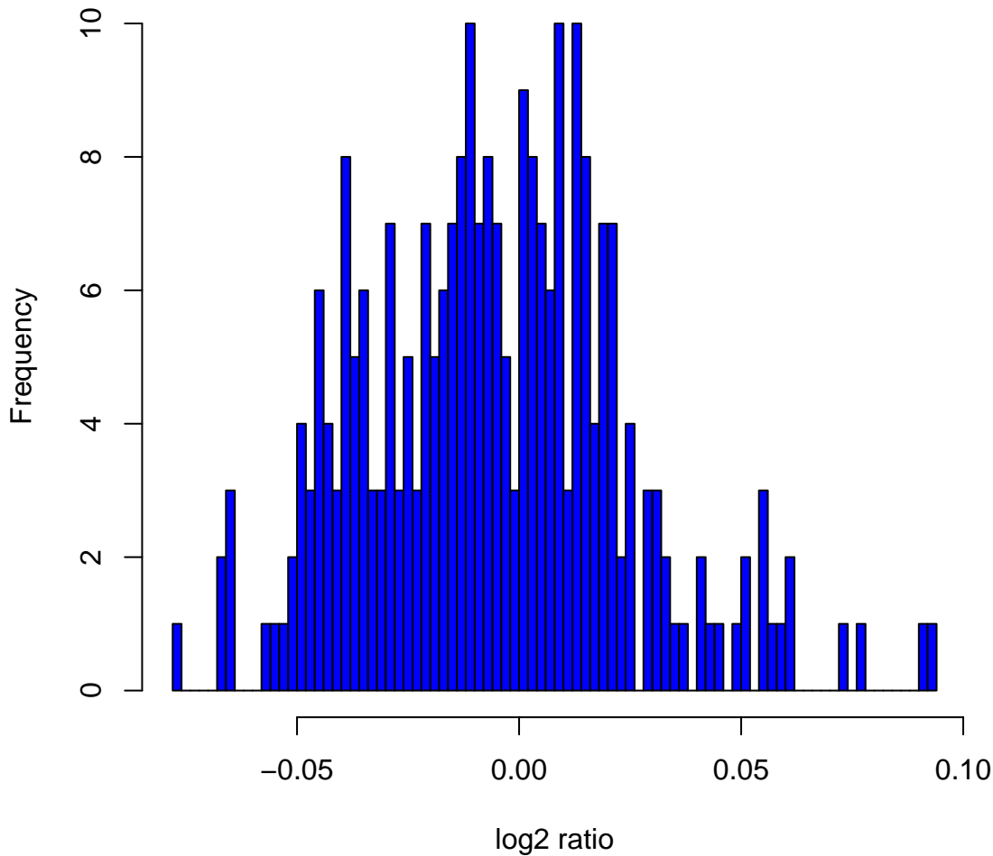
Histogram of log 2 ratios in 270 HapMap samples at clone Chr12tp-7D7
