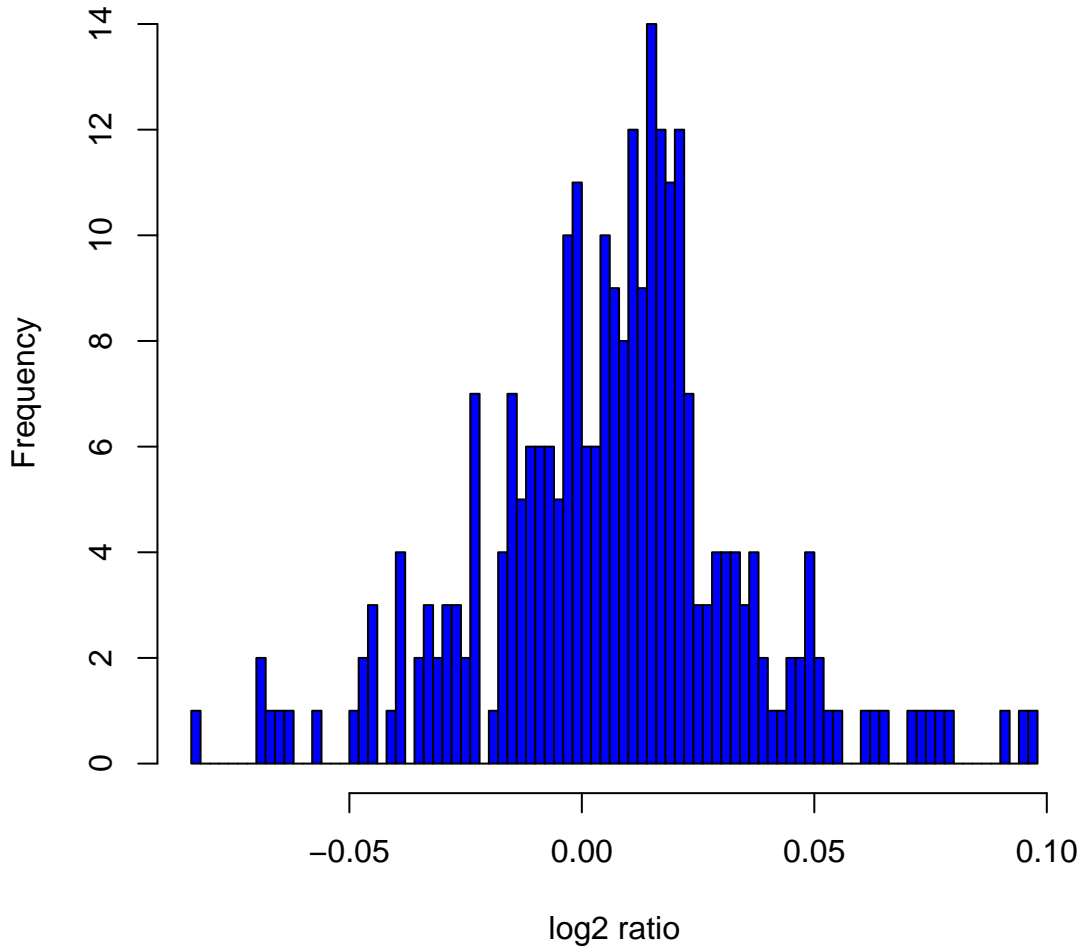
Histogram of log2ratios in 270 HapMap samples at clone Chr12tp-8A11
