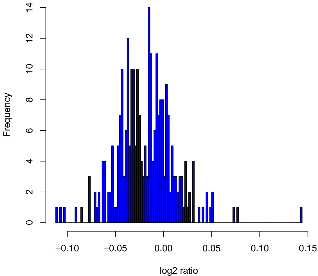
Histogram of log 2 ratios in 270 HapMap samples at clone Chr12tp-8A6
