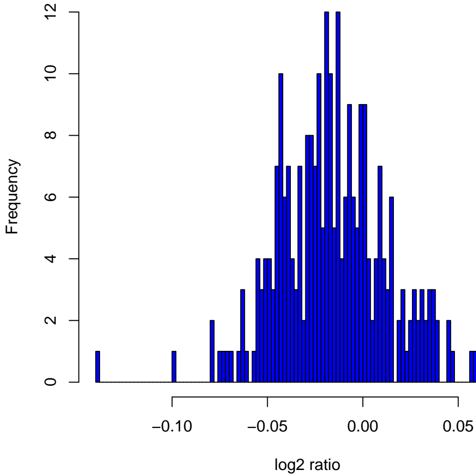
Histogram of log 2 ratios in 270 HapMap samples at clone Chr12tp-8B7
