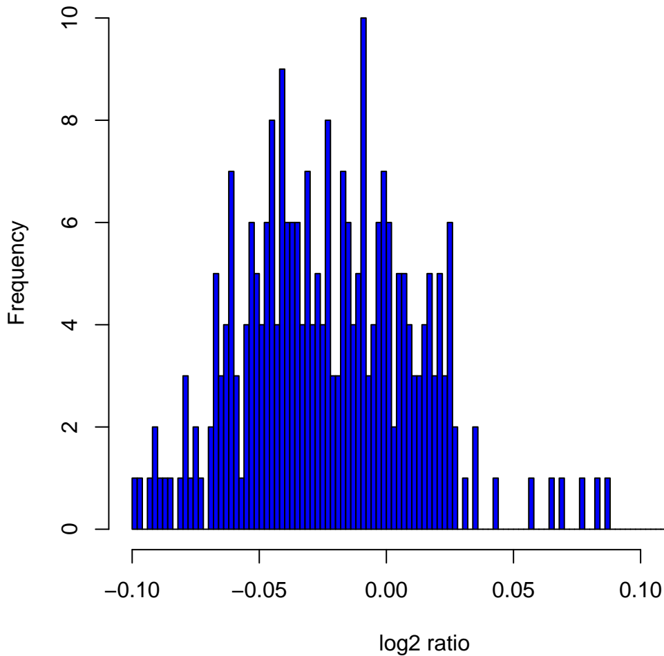
Histogram of log 2 ratios in 270 HapMap samples at clone Chr12tp-8D9
