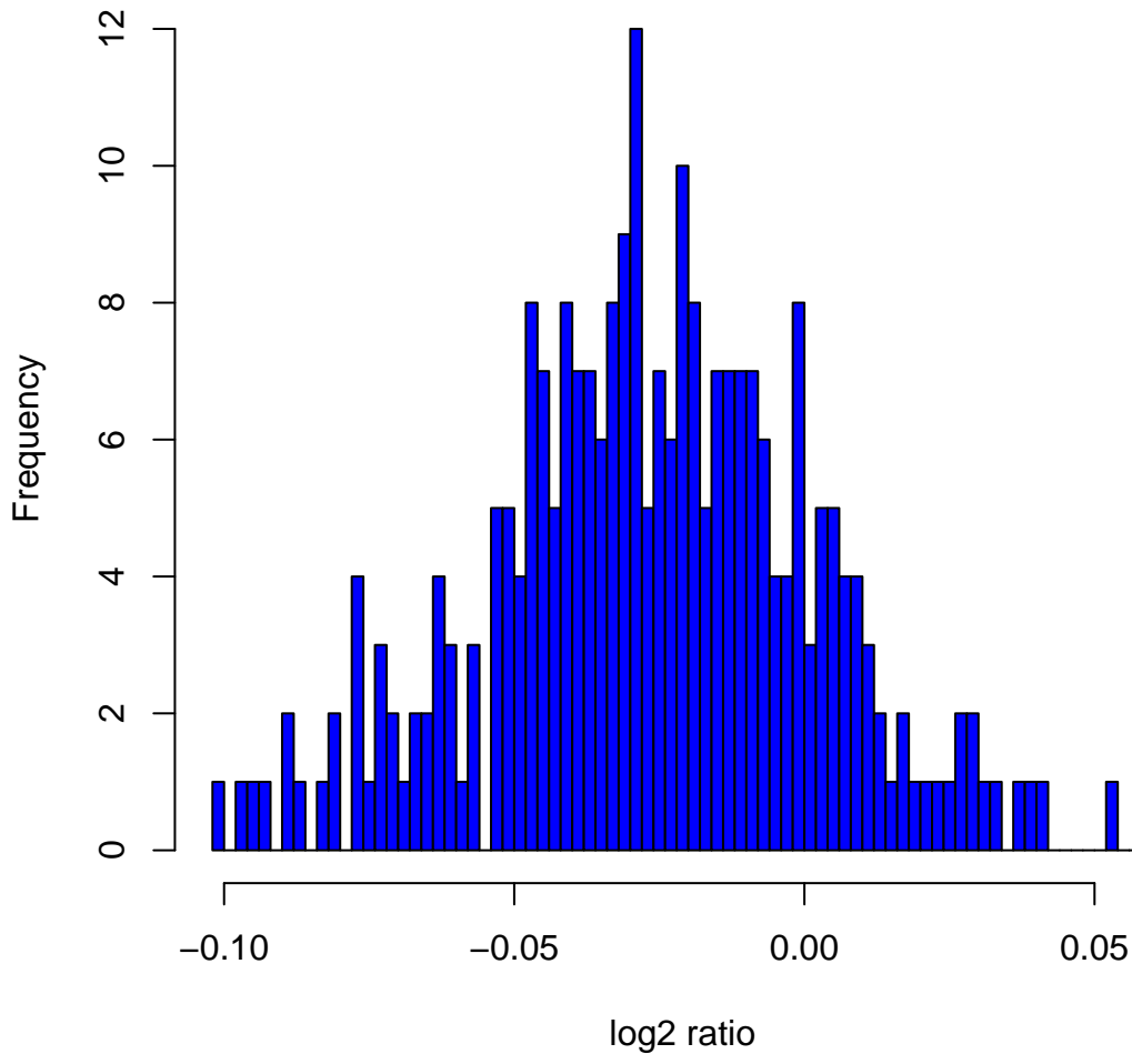
Histogram of log 2 ratios in 270 HapMap samples at clone Chr12tp-8E9
