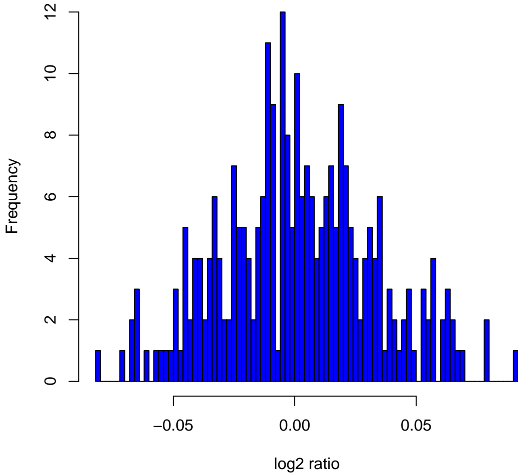
Histogram of log 2 ratios in 270 HapMap samples at clone Chr12tp-8G8
