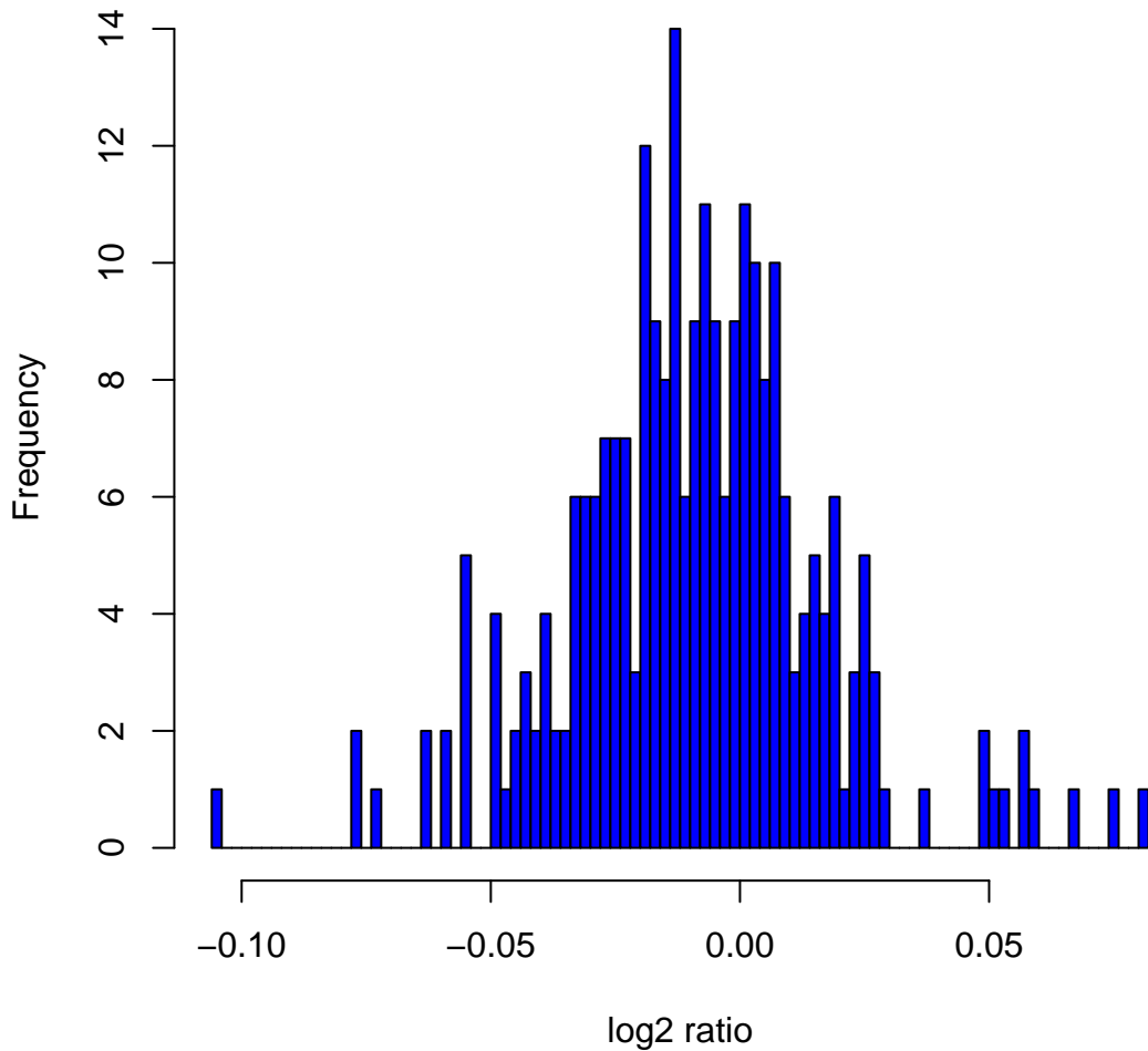
Histogram of log 2 ratios in 270 HapMap samples at clone Chr12tp-9H7
