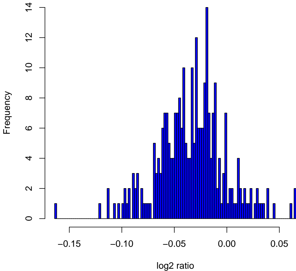
Histogram of log 2 ratios in 270 HapMap samples at clone Chr5tp-23D3
