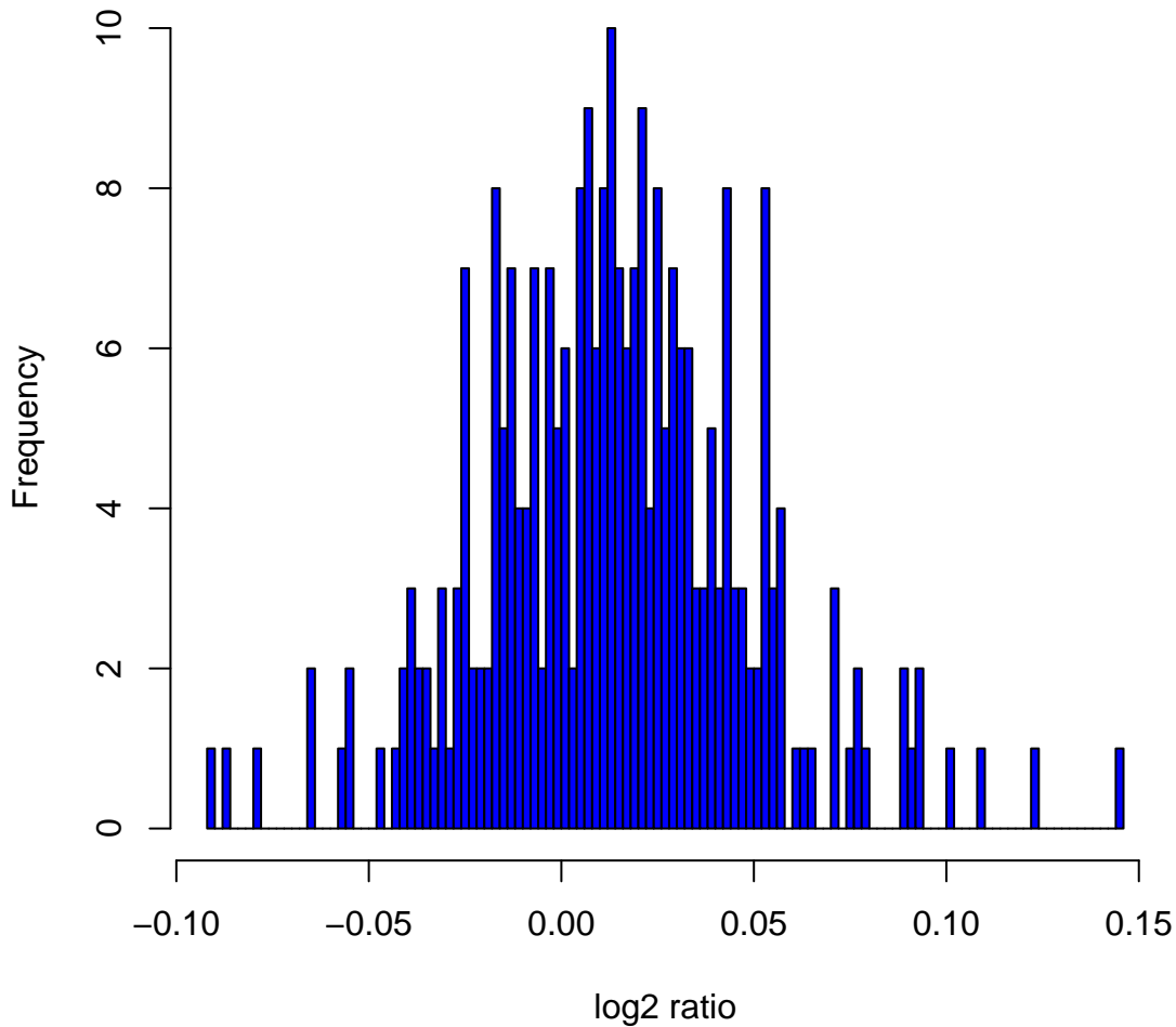
Histogram of log2ratios in 270 HapMap samples at clone Chr6tp-17G10
