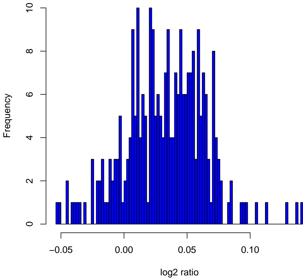
Histogram of log2ratios in 270 HapMap samples at clone Chr13tp-10A10
