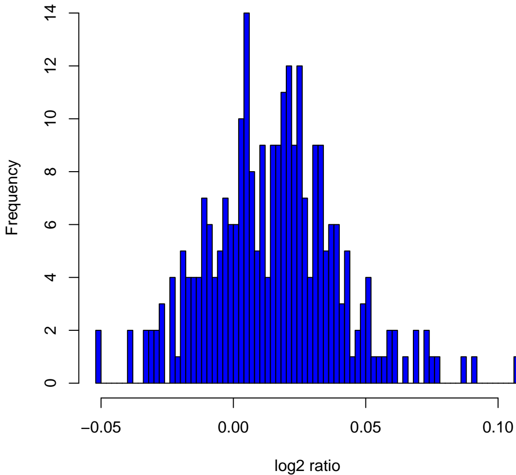
Histogram of \log_2 ratios in 270 HapMap samples at clone Chr13tp-10G10
