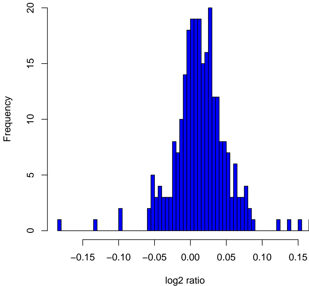
Histogram of log2ratios in 270 HapMap samples at clone Chr13tp-10G9
