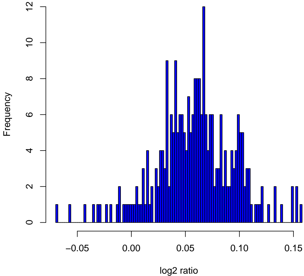
Histogram of log2ratios in 270 HapMap samples at clone Chr13tp-11B3
