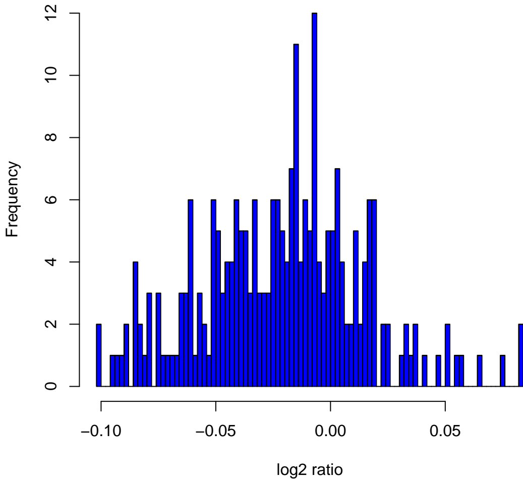
Histogram of log2ratios in 270 HapMap samples at clone Chr13tp-11B6
