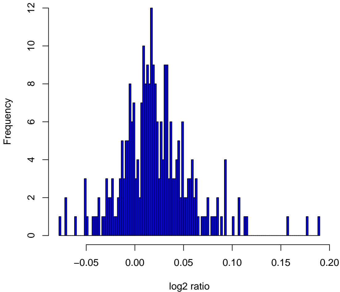
Histogram of log2ratios in 270 HapMap samples at clone Chr13tp-11D6
