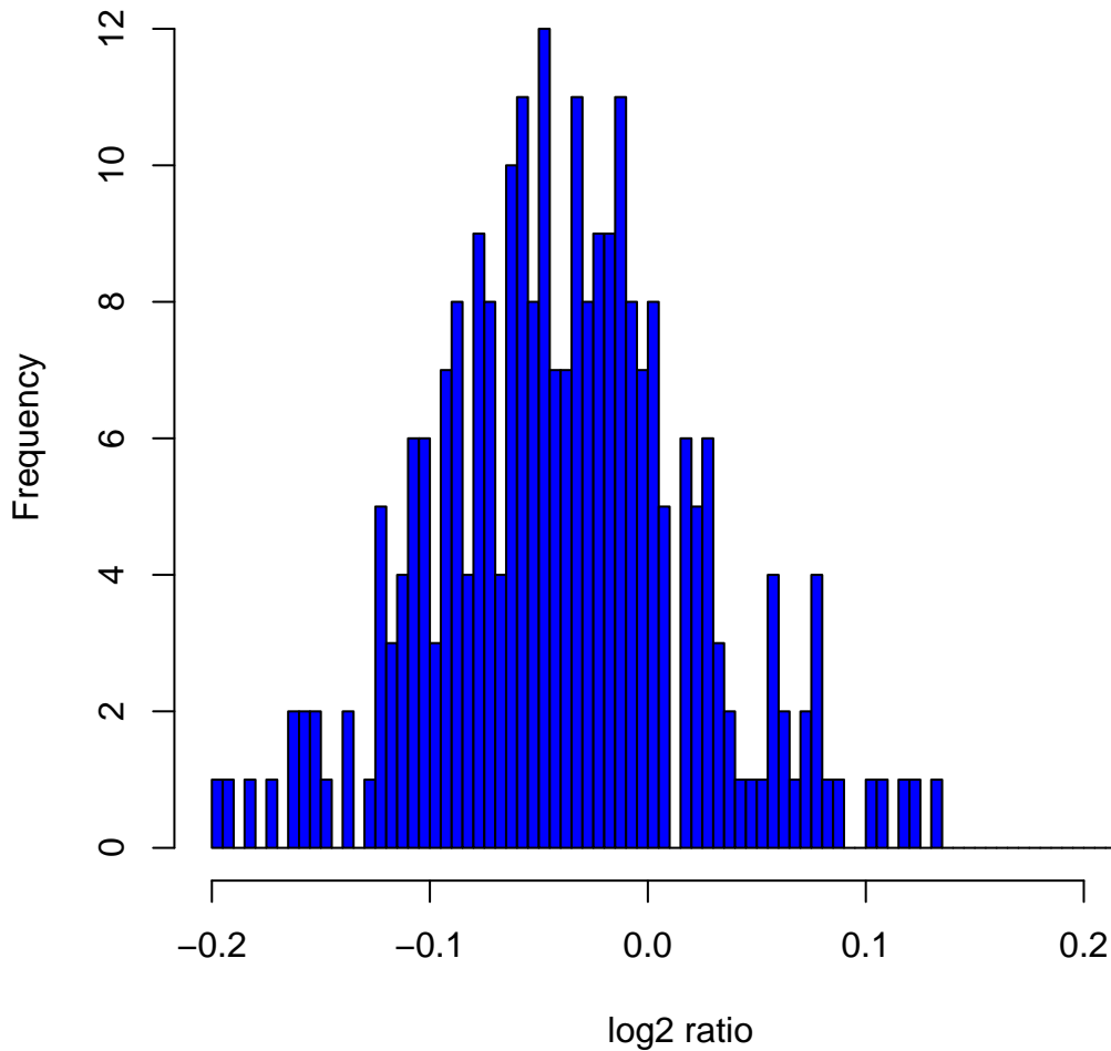
Histogram of log 2 ratios in 270 HapMap samples at clone Chr13tp-1D9
