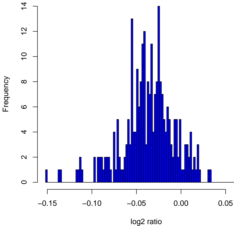
Histogram of log2ratios in 270 HapMap samples at clone Chr13tp-1E10
