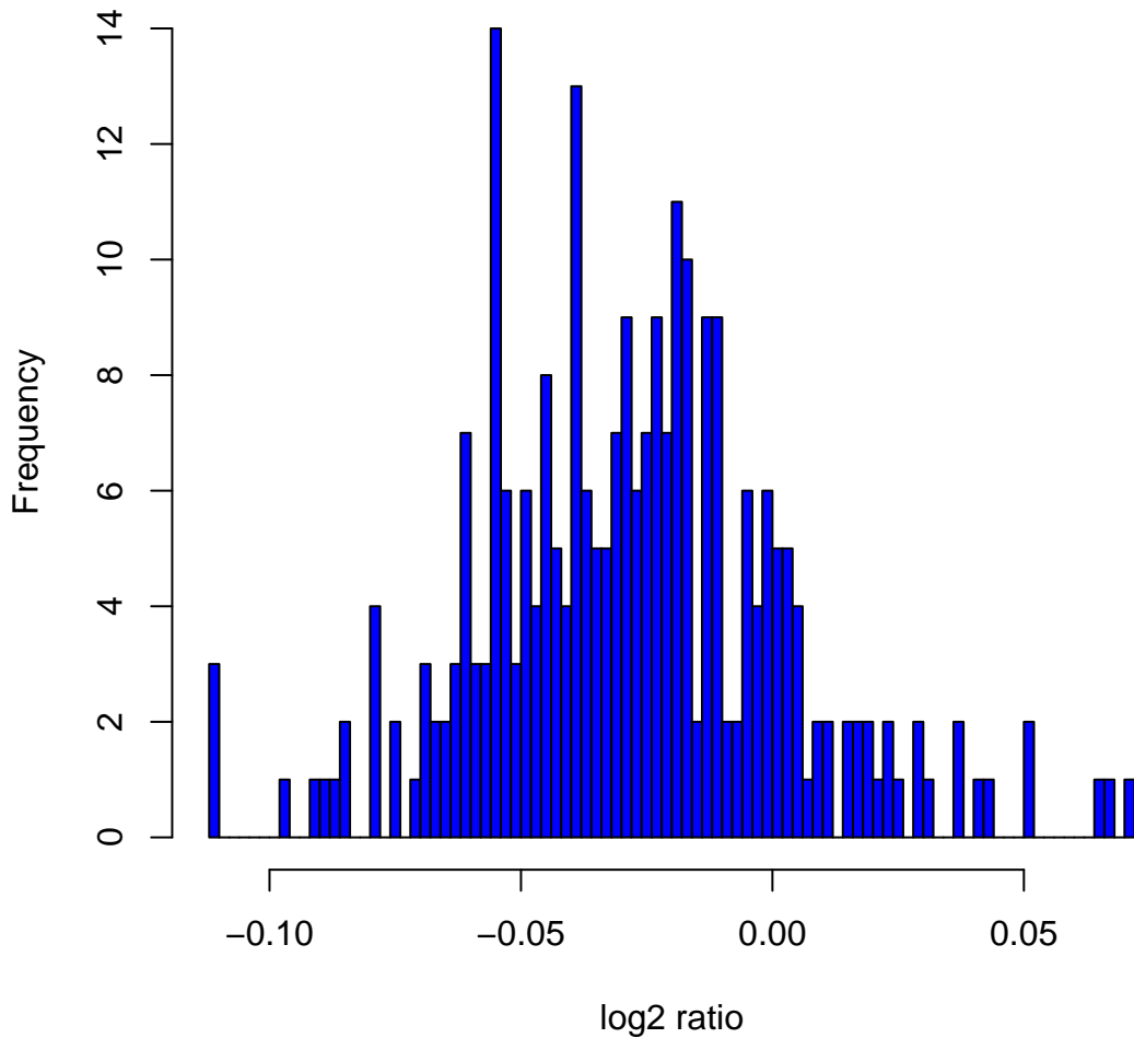
Histogram of log 2 ratios in 270 HapMap samples at clone Chr13tp-1G7
