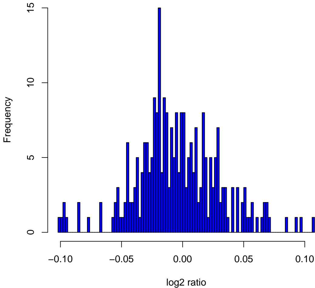
Histogram of log 2 ratios in 270 HapMap samples at clone Chr13tp-1H2
