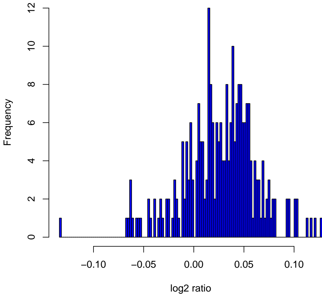
Histogram of log 2 ratios in 270 HapMap samples at clone Chr13tp-3B1
