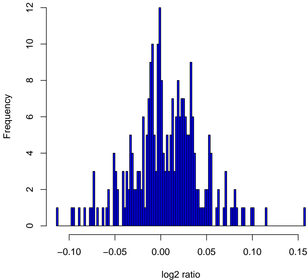
Histogram of log 2 ratios in 270 HapMap samples at clone Chr13tp-3B9
