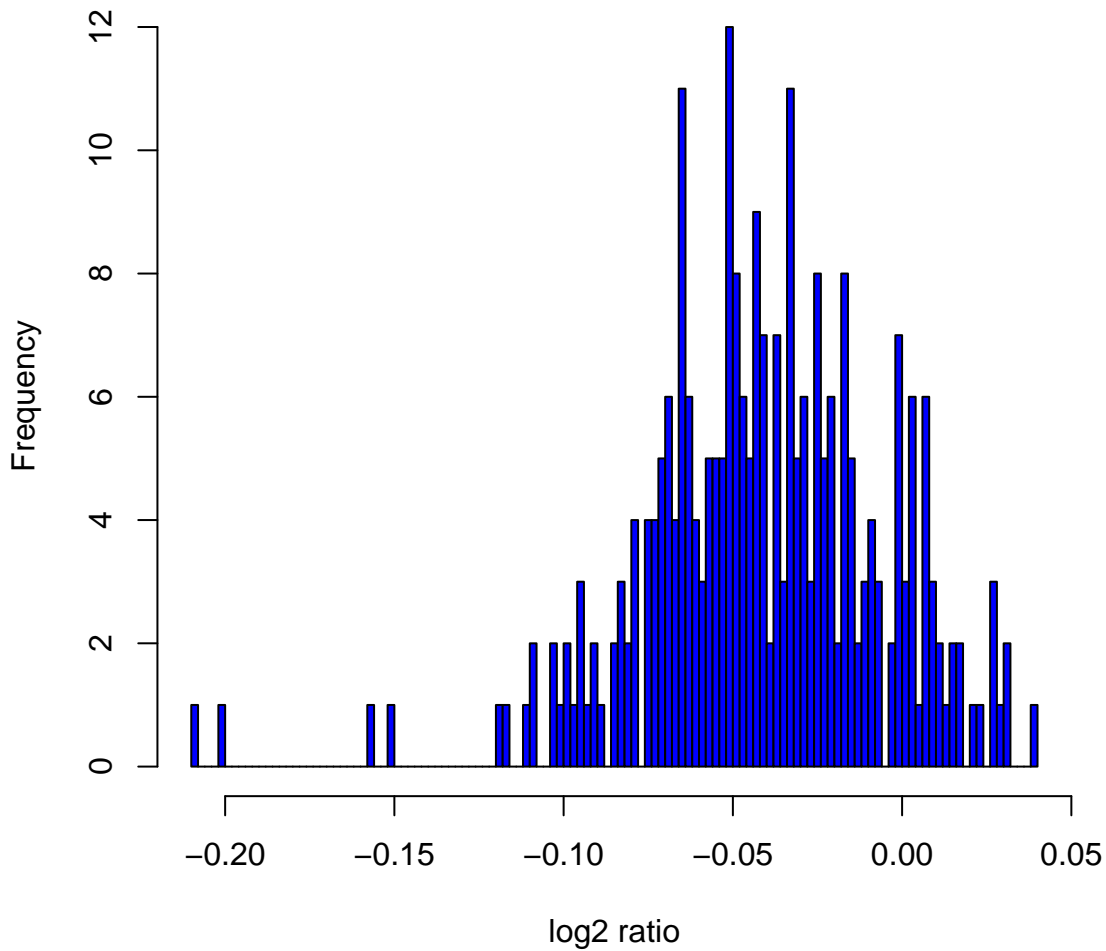
Histogram of log2ratios in 270 HapMap samples at clone Chr13tp-3C7
