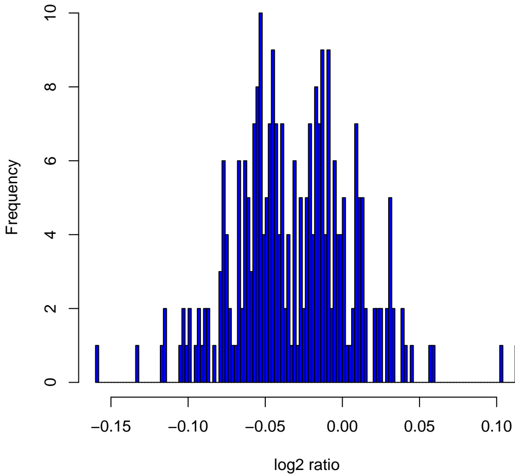
Histogram of log 2 ratios in 270 HapMap samples at clone Chr13tp-3E4
