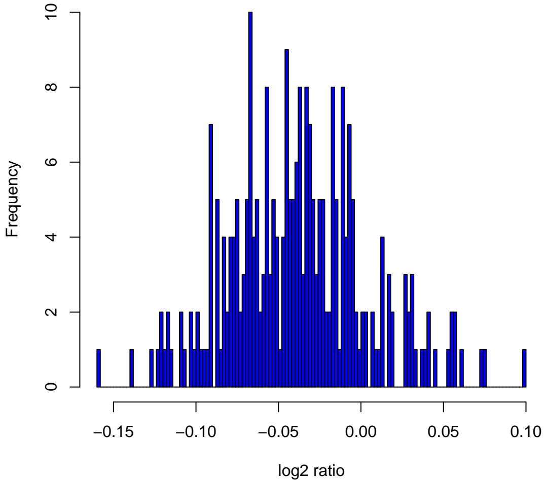
Histogram of log2ratios in 270 HapMap samples at clone Chr13tp-4A11
