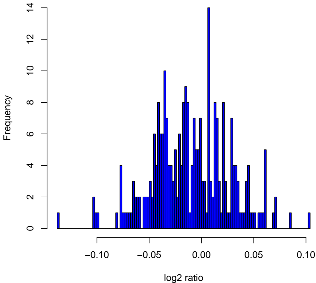
Histogram of log2ratios in 270 HapMap samples at clone Chr13tp-4B10
