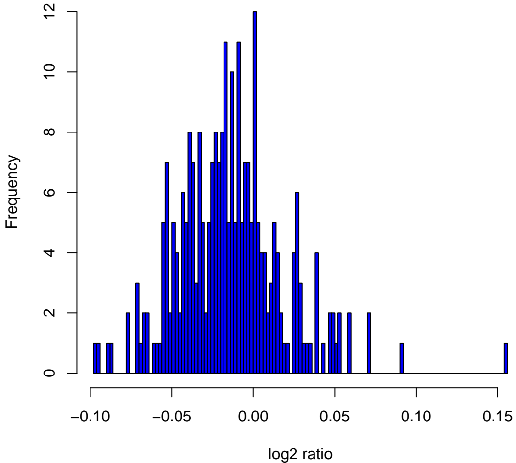
Histogram of log2ratios in 270 HapMap samples at clone Chr13tp-4C11
