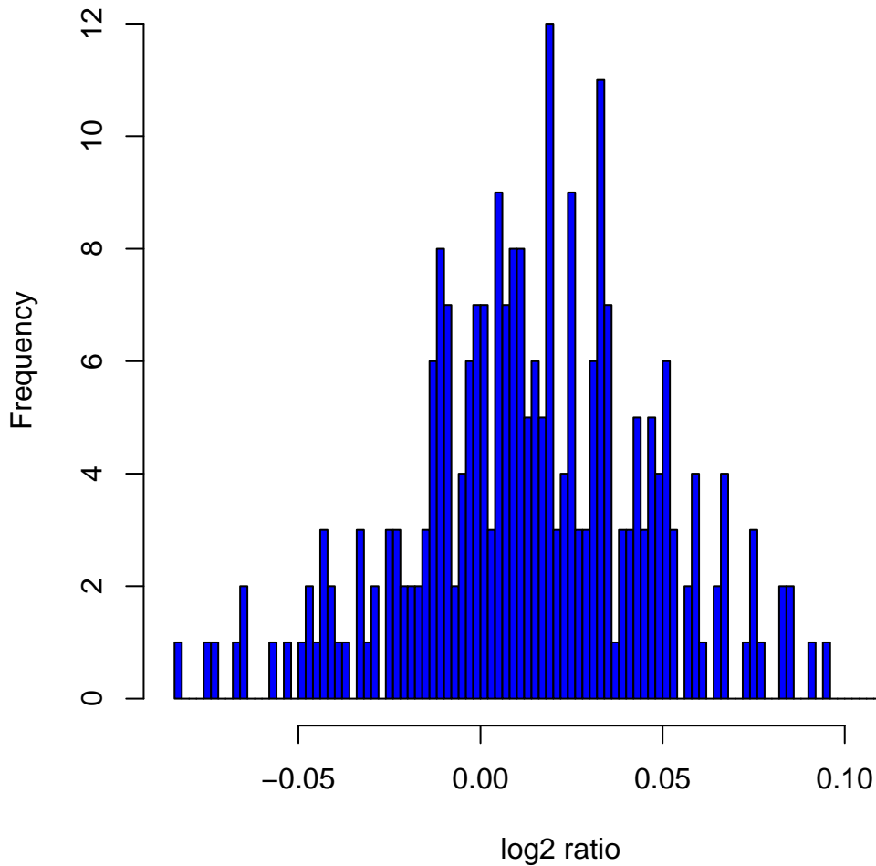
Histogram of log2ratios in 270 HapMap samples at clone Chr13tp-5B10
