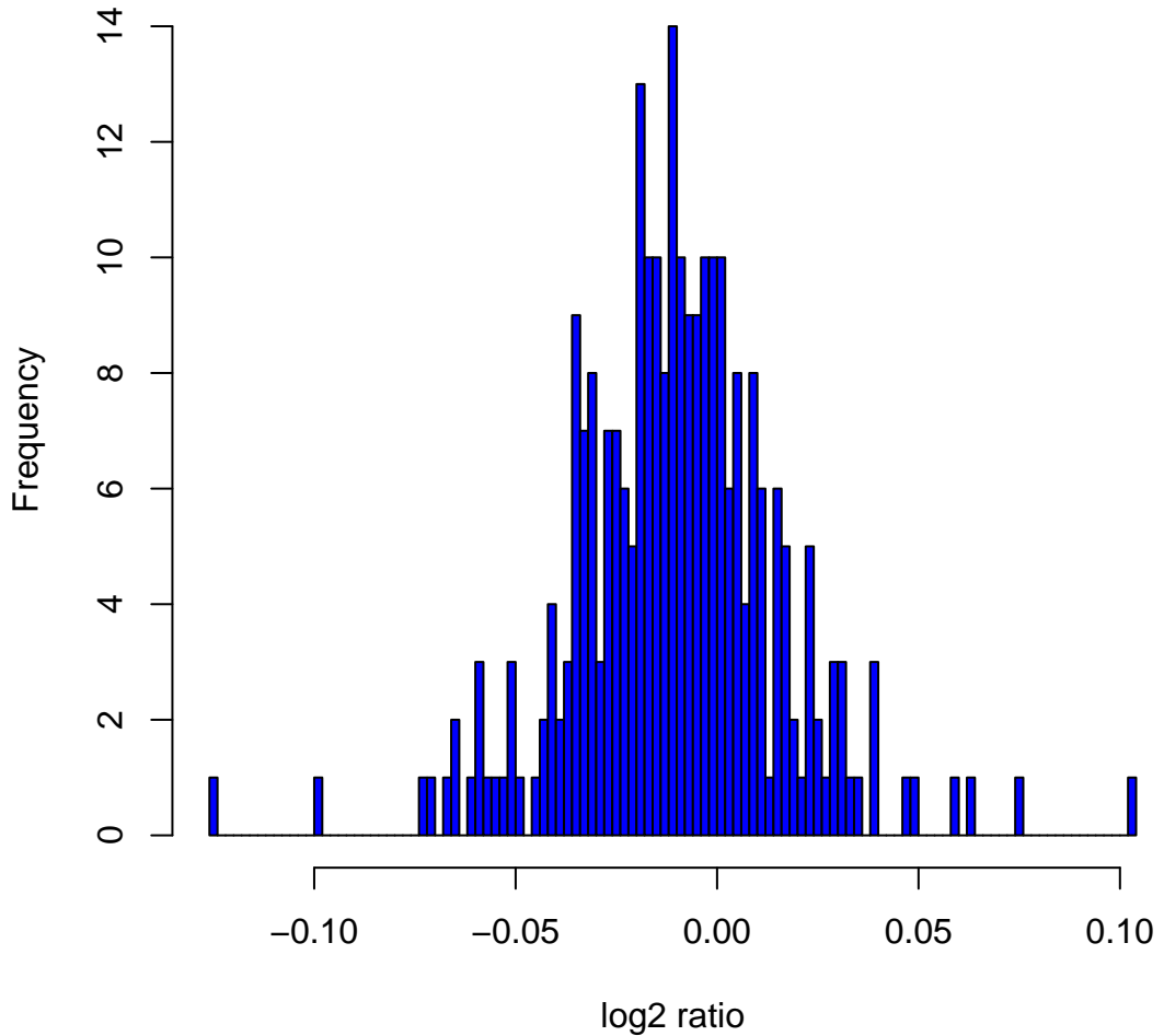
Histogram of log2ratios in 270 HapMap samples at clone Chr13tp-5C11
