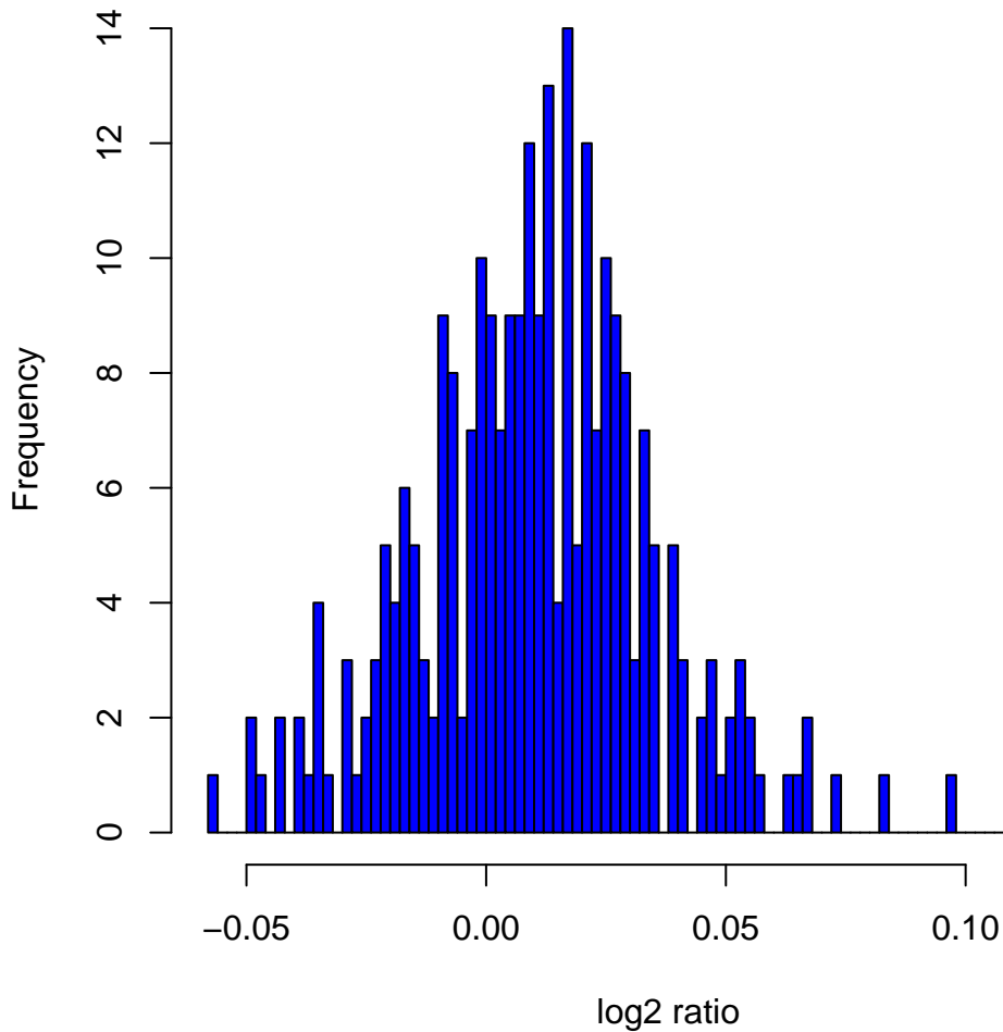
Histogram of log 2 ratios in 270 HapMap samples at clone Chr13tp-5E3
