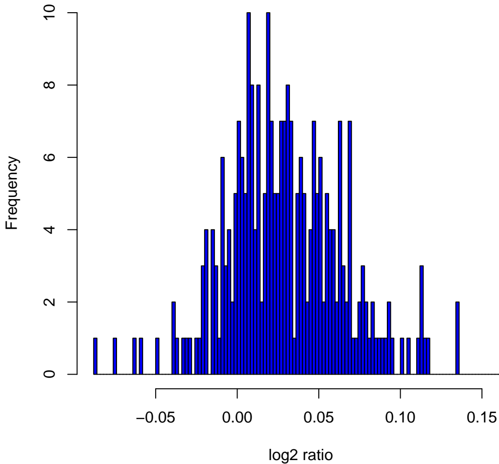
Histogram of log2ratios in 270 HapMap samples at clone Chr13tp-6A10
