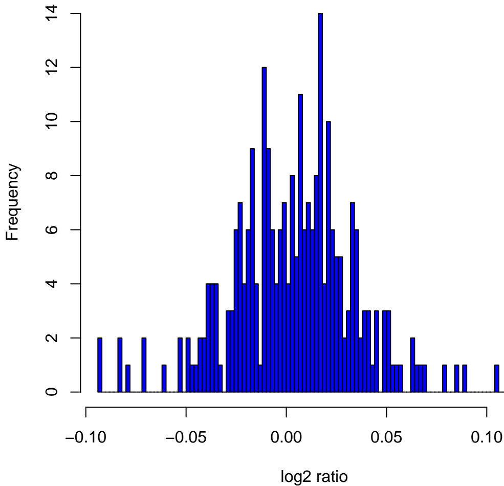
Histogram of log 2 ratios in 270 HapMap samples at clone Chr13tp-6C2
