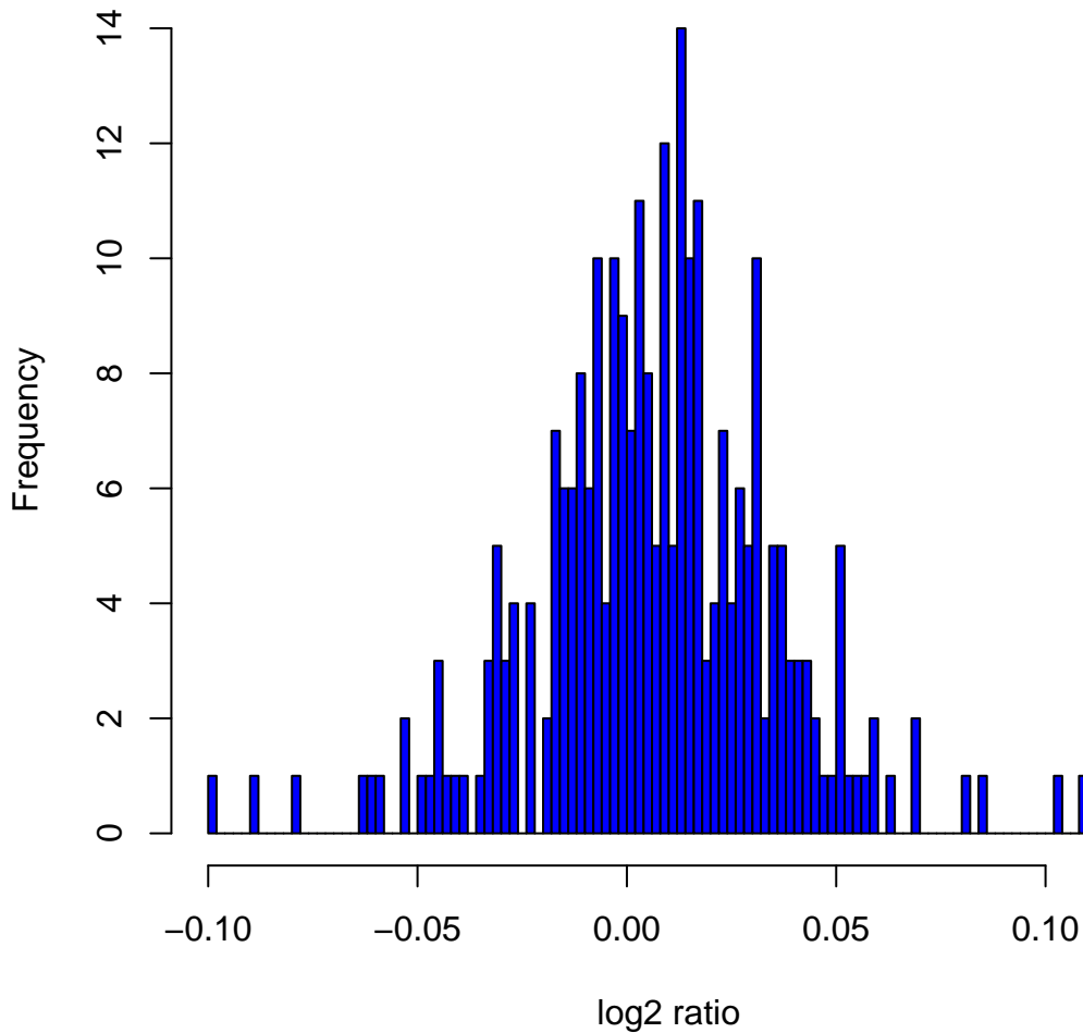
Histogram of log2ratios in 270 HapMap samples at clone Chr13tp-6C8
