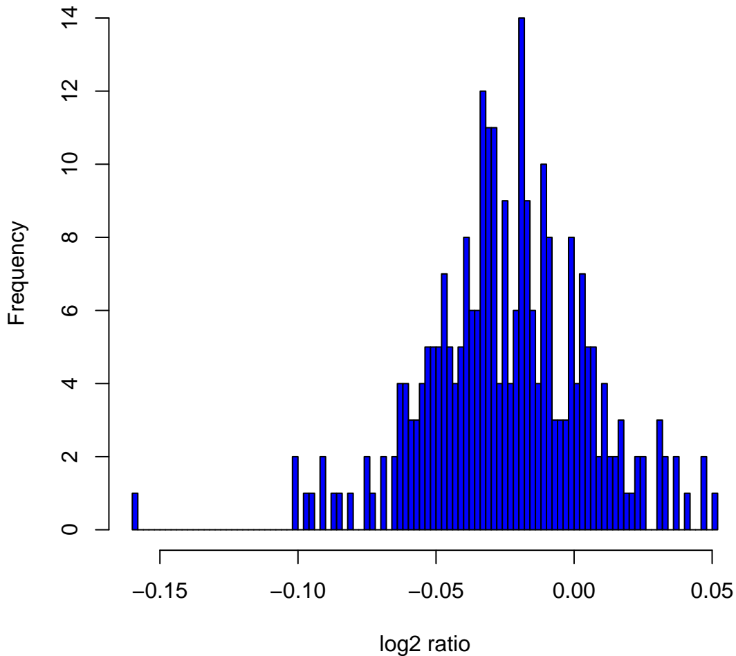
Histogram of log2ratios in 270 HapMap samples at clone Chr13tp-6E1
