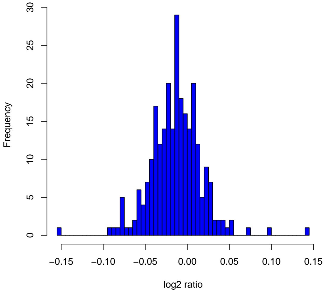
Histogram of log2ratios in 270 HapMap samples at clone Chr13tp-6F1
