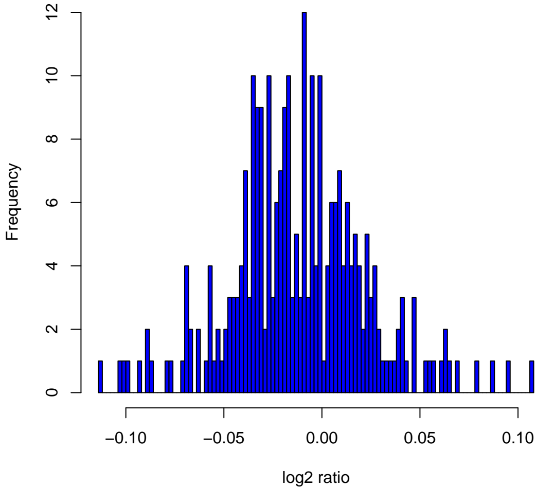
Histogram of log2ratios in 270 HapMap samples at clone Chr13tp-6F10
