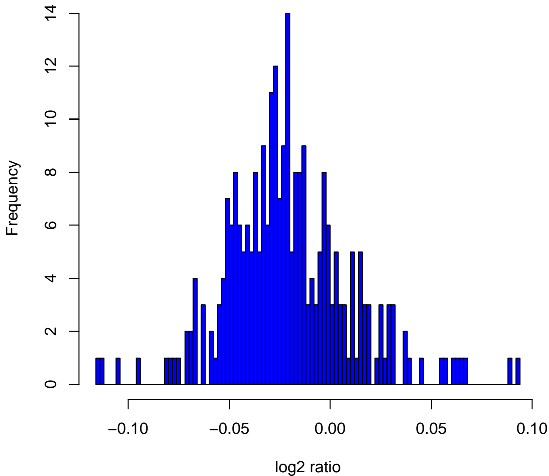
Histogram of log2ratios in 270 HapMap samples at clone Chr13tp-6G9
