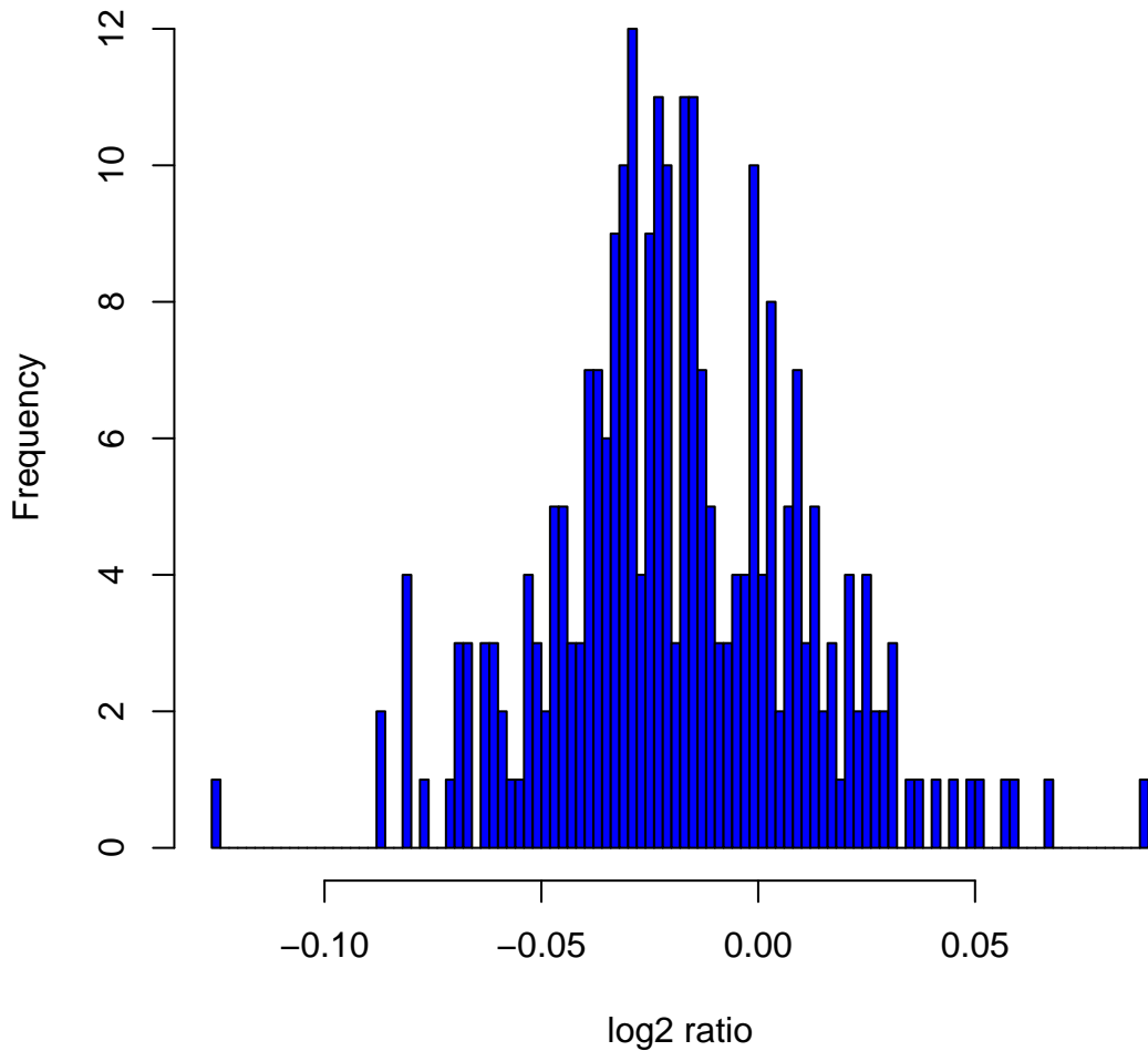
Histogram of log2ratios in 270 HapMap samples at clone Chr13tp-7B10
