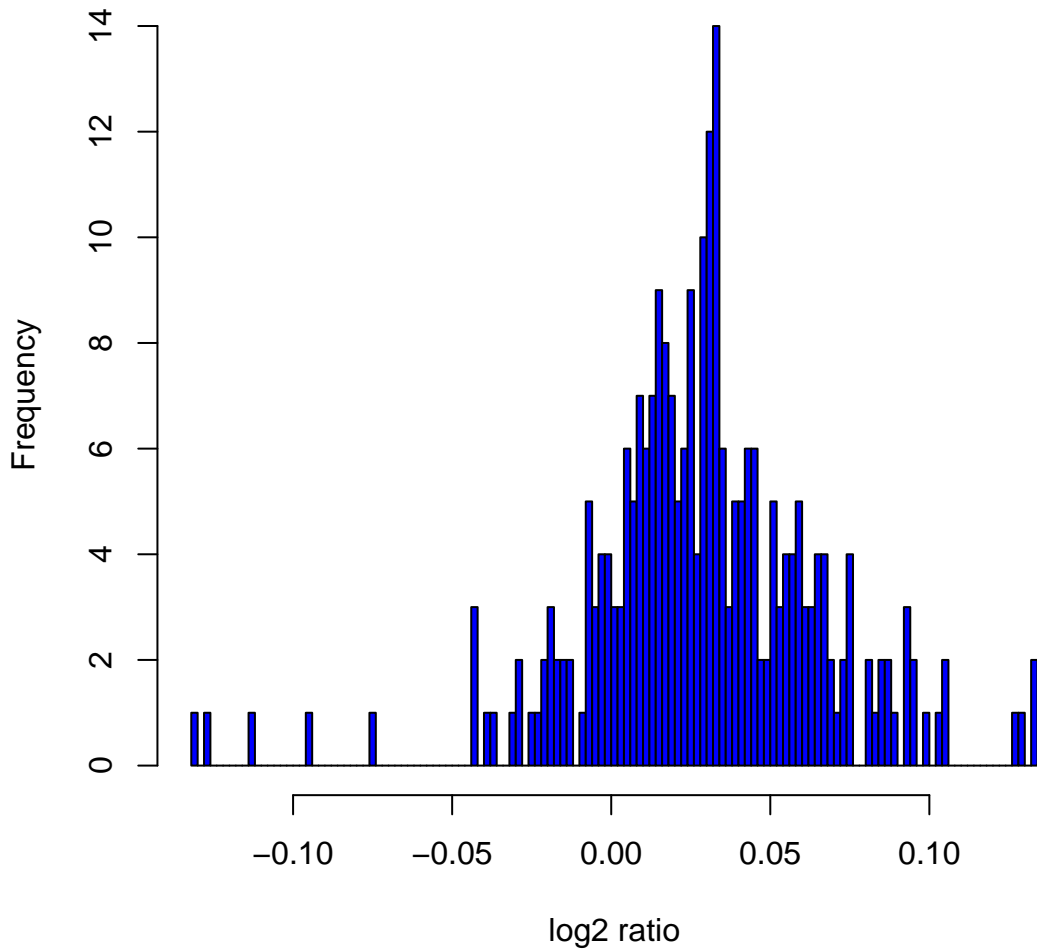
Histogram of log2ratios in 270 HapMap samples at clone Chr13tp-7C10
