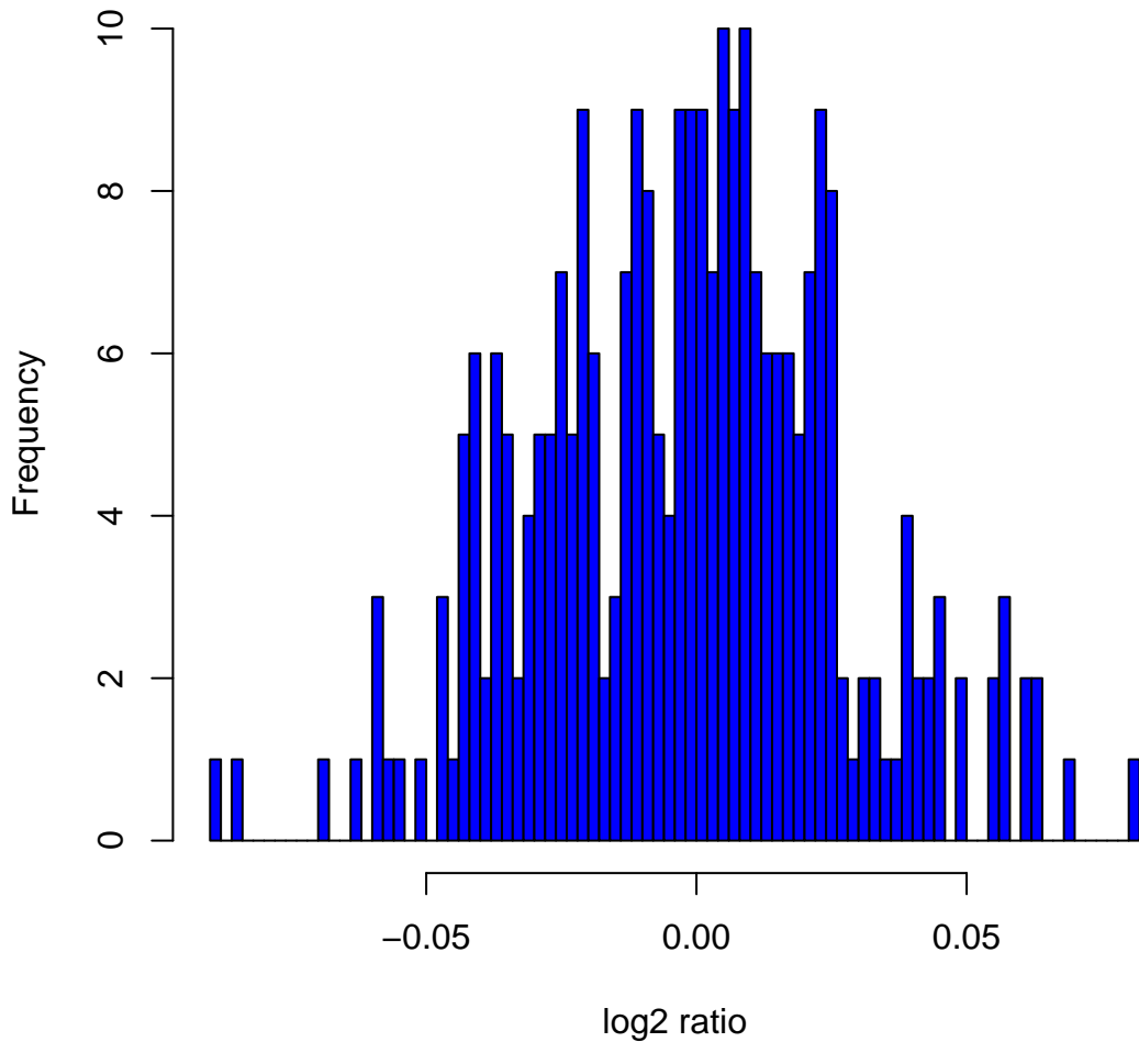
Histogram of log2ratios in 270 HapMap samples at clone Chr13tp-7C12
