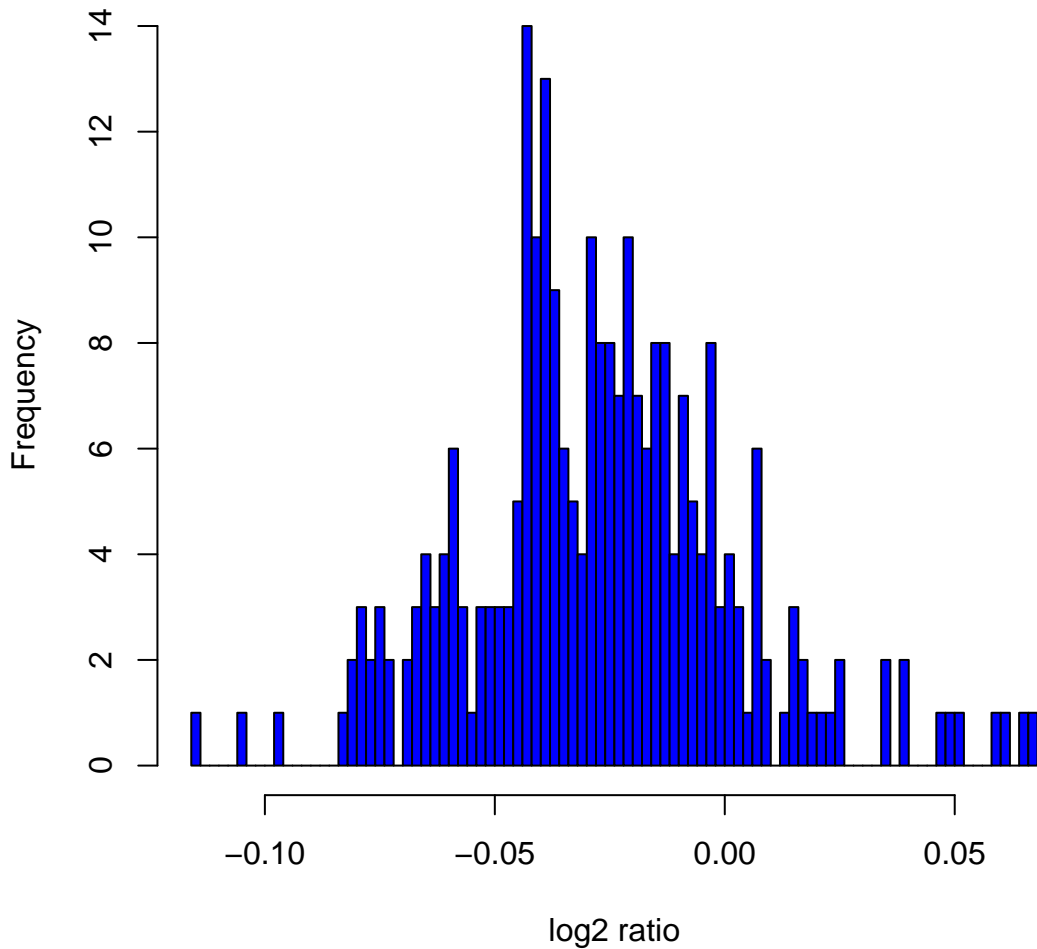
Histogram of log 2 ratios in 270 HapMap samples at clone Chr13tp-7G1
