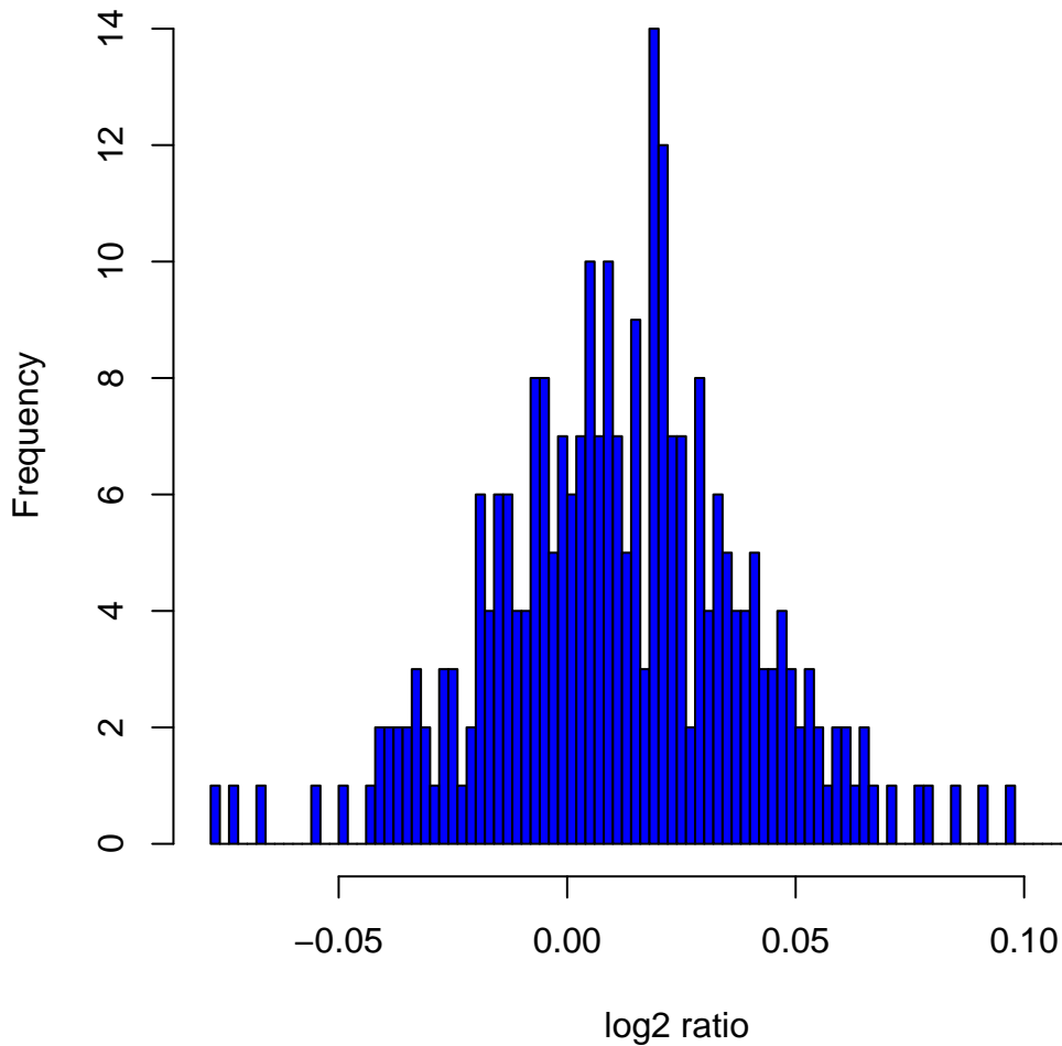
Histogram of log2ratios in 270 HapMap samples at clone Chr13tp-8B8
