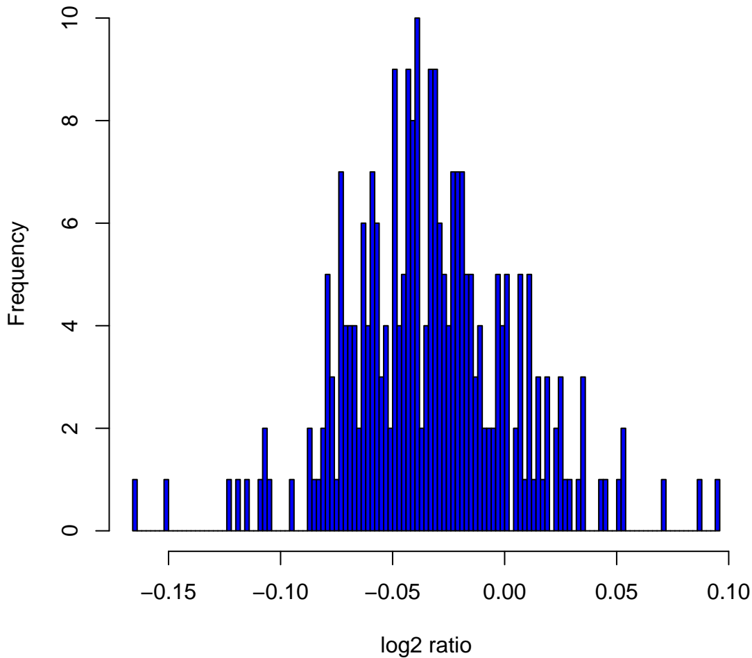
Histogram of log2ratios in 270 HapMap samples at clone Chr13tp-8C12
