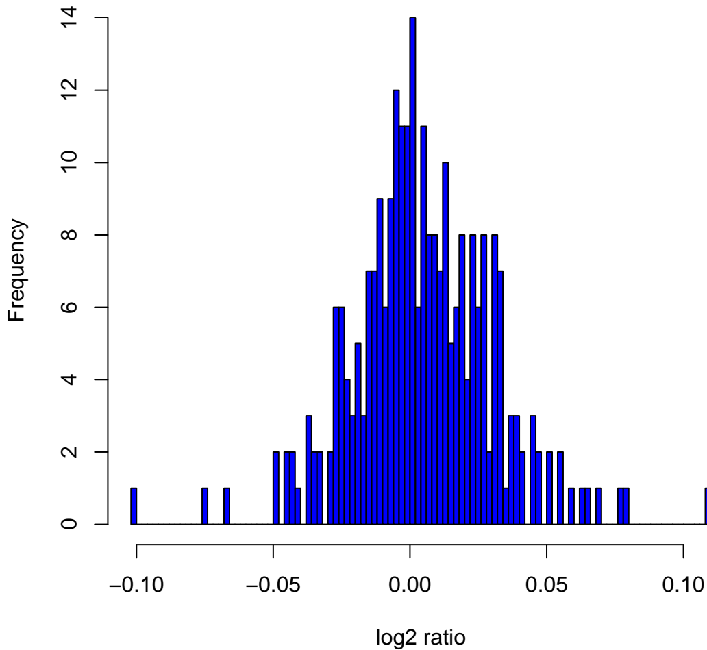
Histogram of log 2 ratios in 270 HapMap samples at clone Chr13tp-8C9
