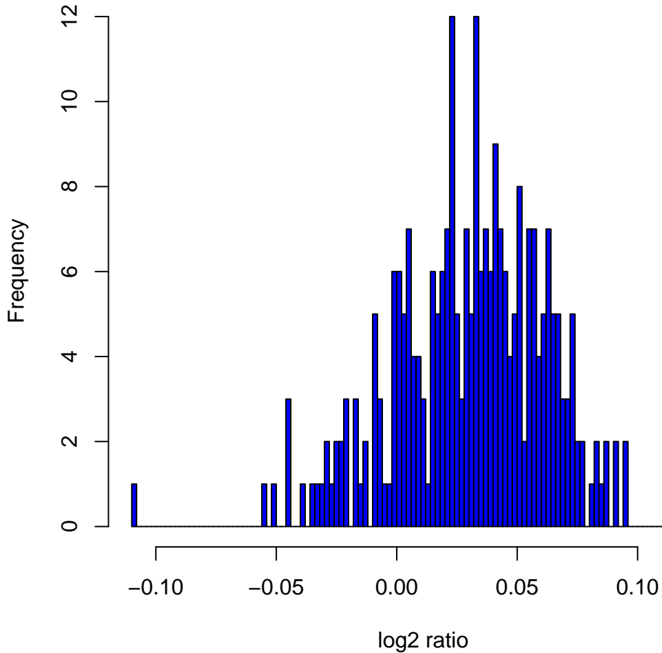
Histogram of log 2 ratios in 270 HapMap samples at clone Chr13tp-8D2
