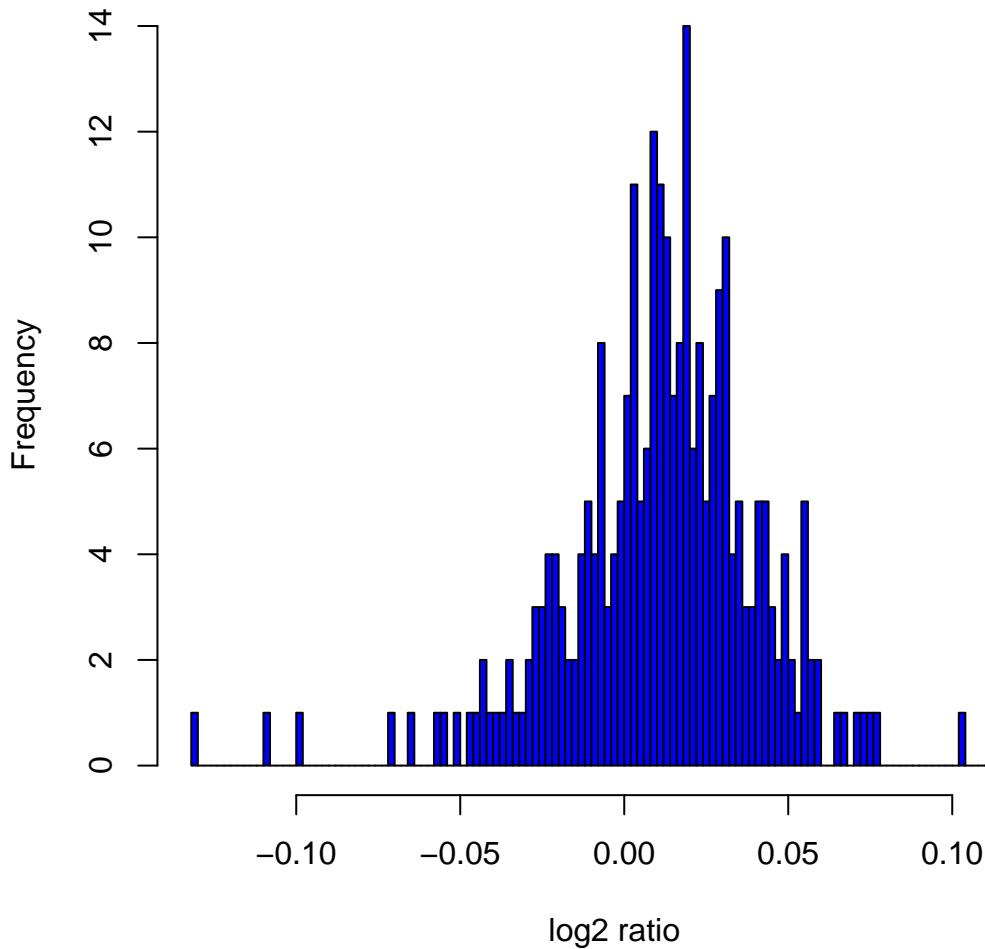
Histogram of log2ratios in 270 HapMap samples at clone Chr13tp-8G4
