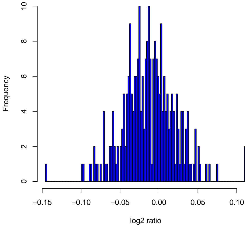
Histogram of \log_2 ratios in 270 HapMap samples at clone Chr13tp-8G5
