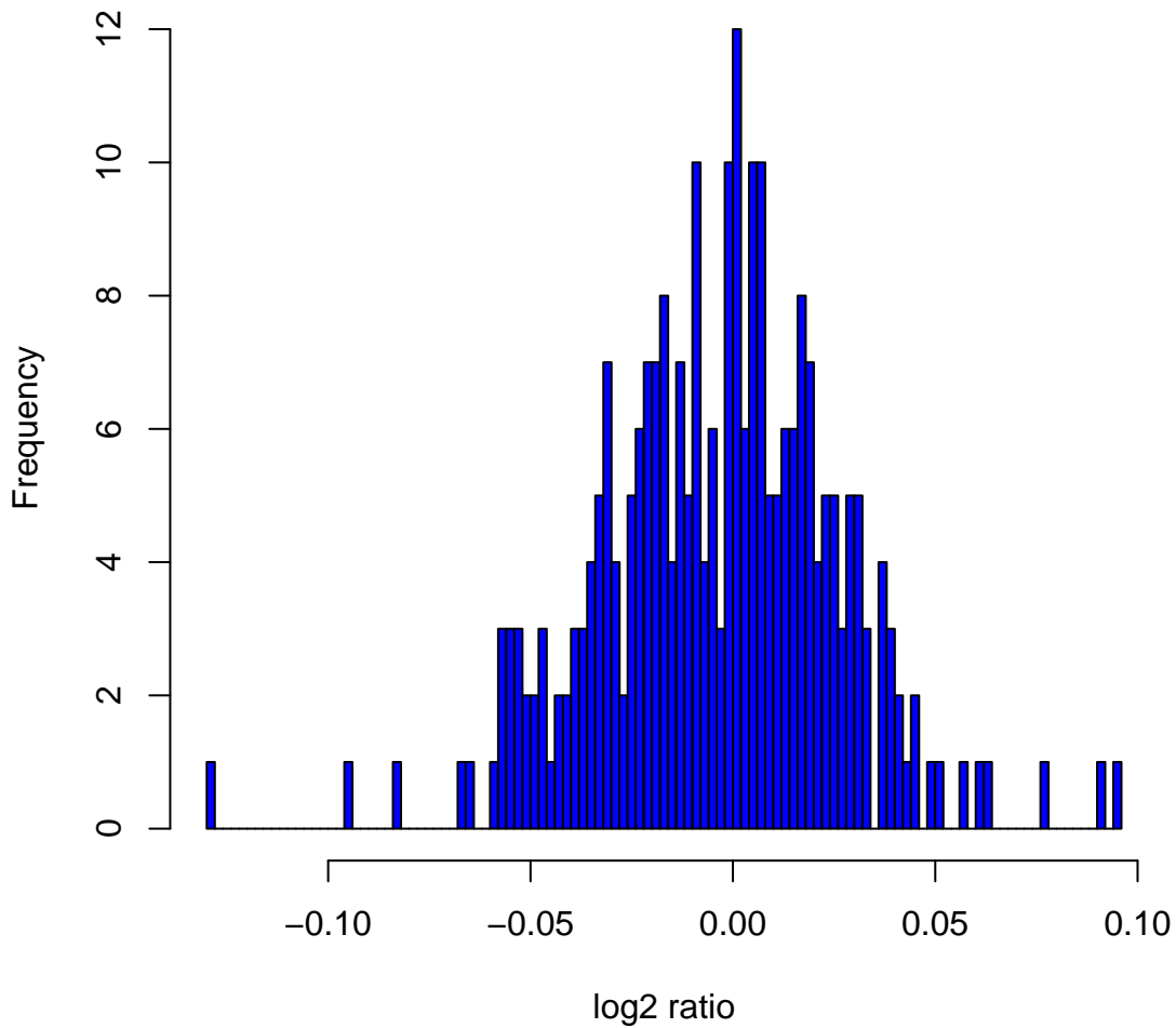
Histogram of log2ratios in 270 HapMap samples at clone Chr13tp-8H4
