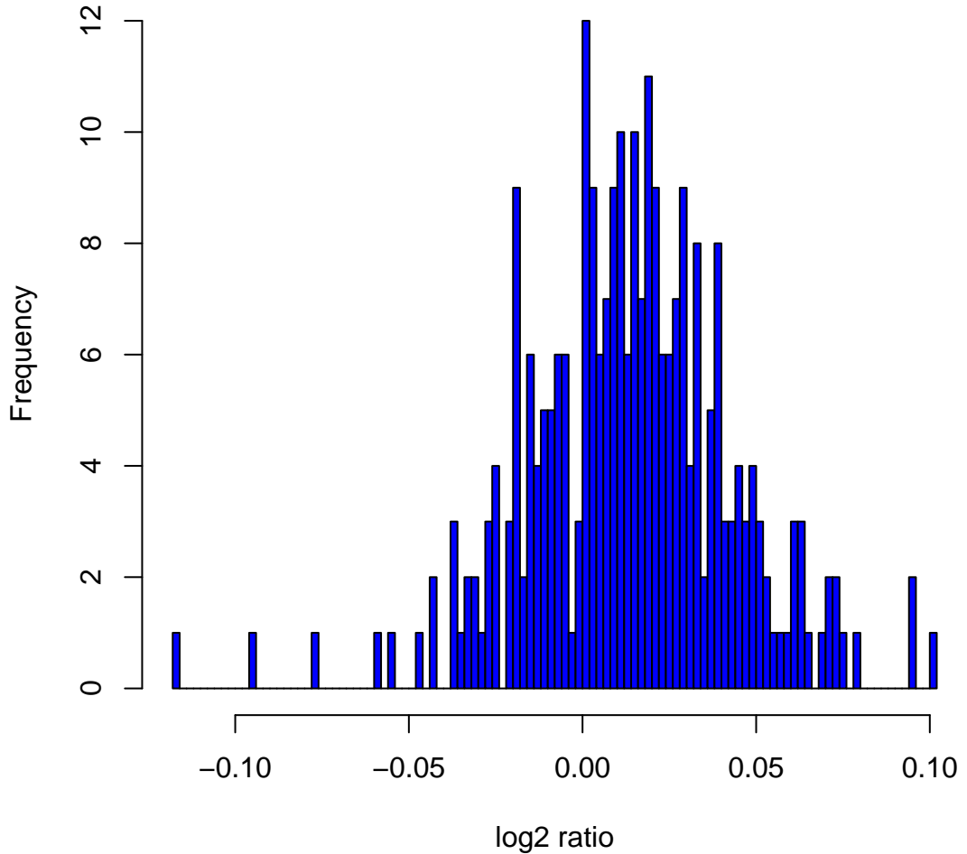
Histogram of log2ratios in 270 HapMap samples at clone Chr13tp-9D11
